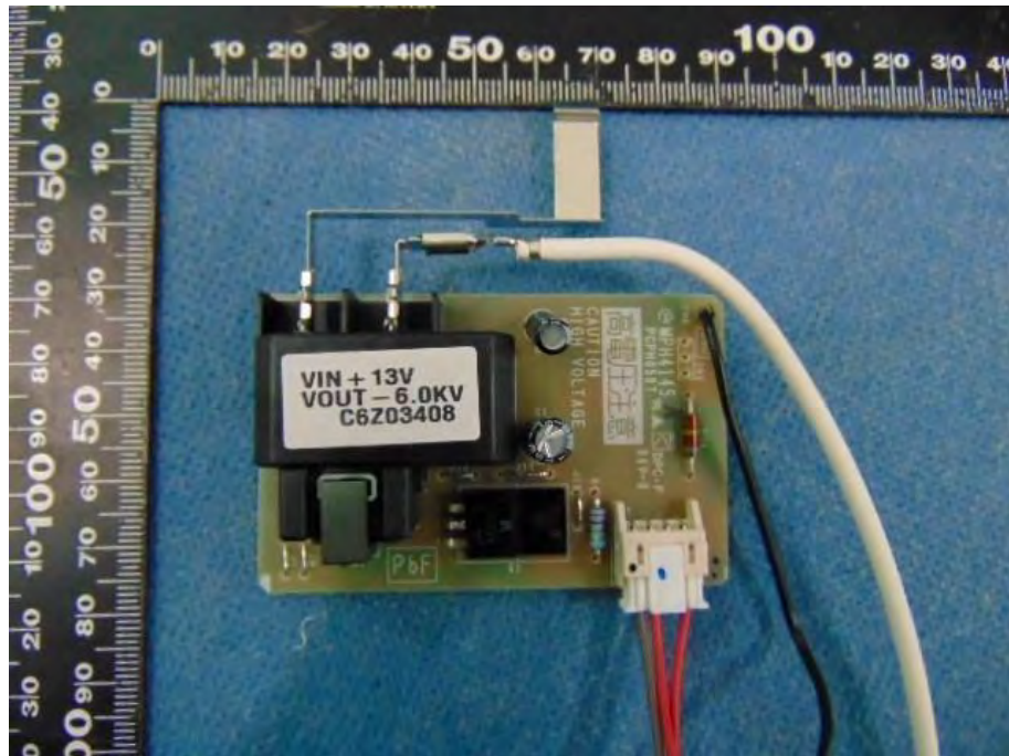
Picture No.17 : Component view of PCB model: MPH4145
