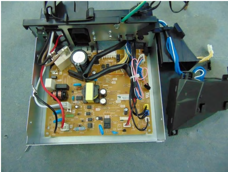
Picture No.41: PCB. compartment of indoor unit: RAS-B10J2KVRG-E
