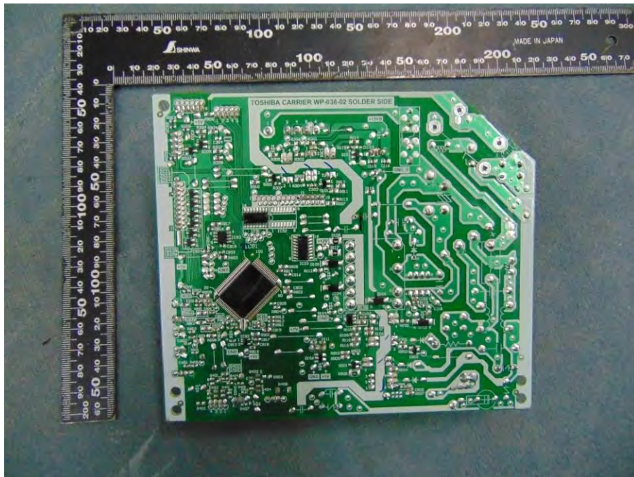
Picture No.67: Pattern view of PCB model: WP-038
