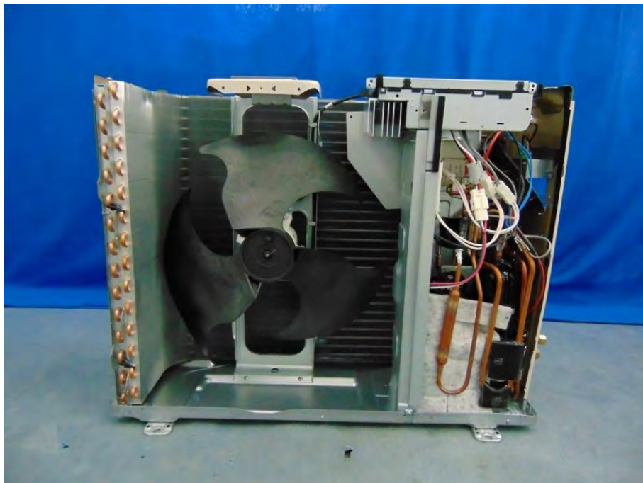
Picture No.32: Inner view of outdoor unit model: RAS-24PAVSG-EE
