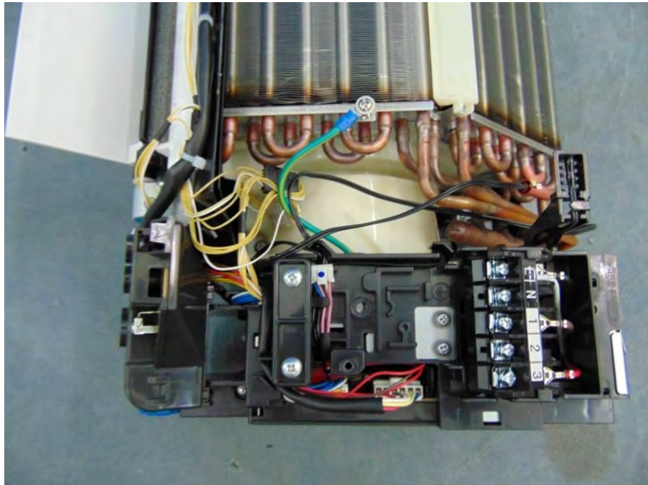
Picture No.52: Terminal view of indoor unit model: RAS-B22J2KVRG-E
