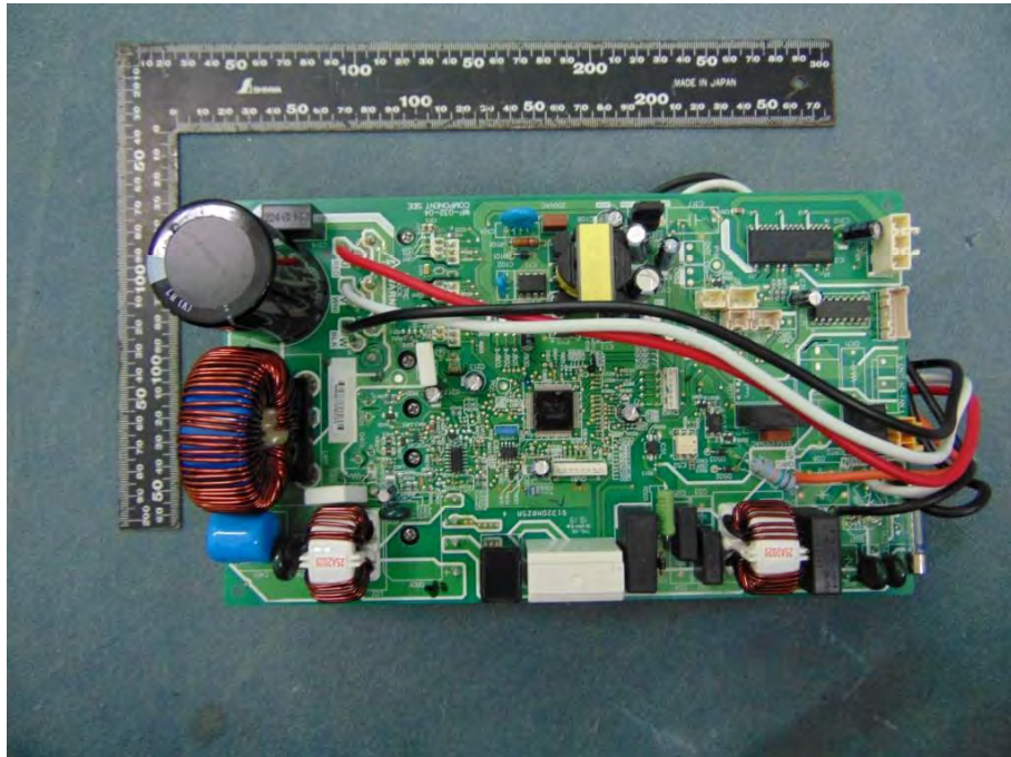
Picture No.72: Component view of PCB model: WP-048
