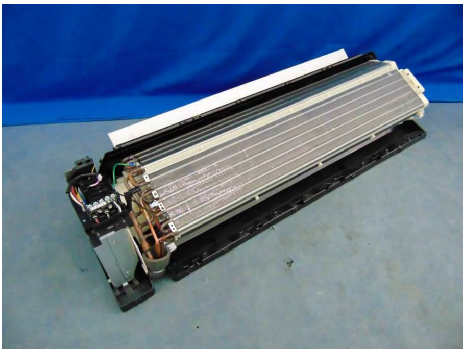
Picture No.63: Overall inner view of indoor unit model: RAS-24PKVSG-EE
