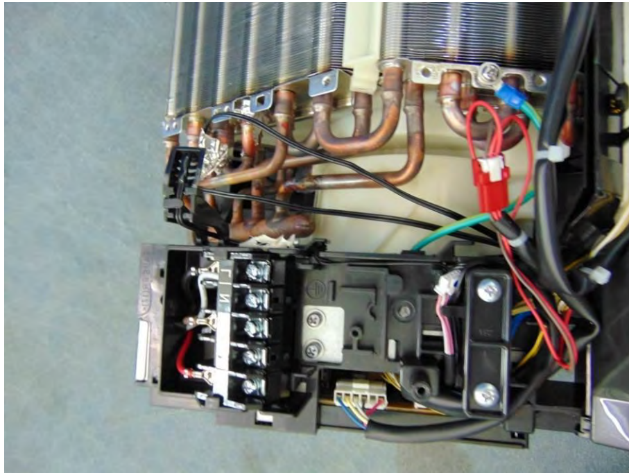
Picture No.58: Terminal view of indoor unit model: RAS-B24J2KVRG-E
