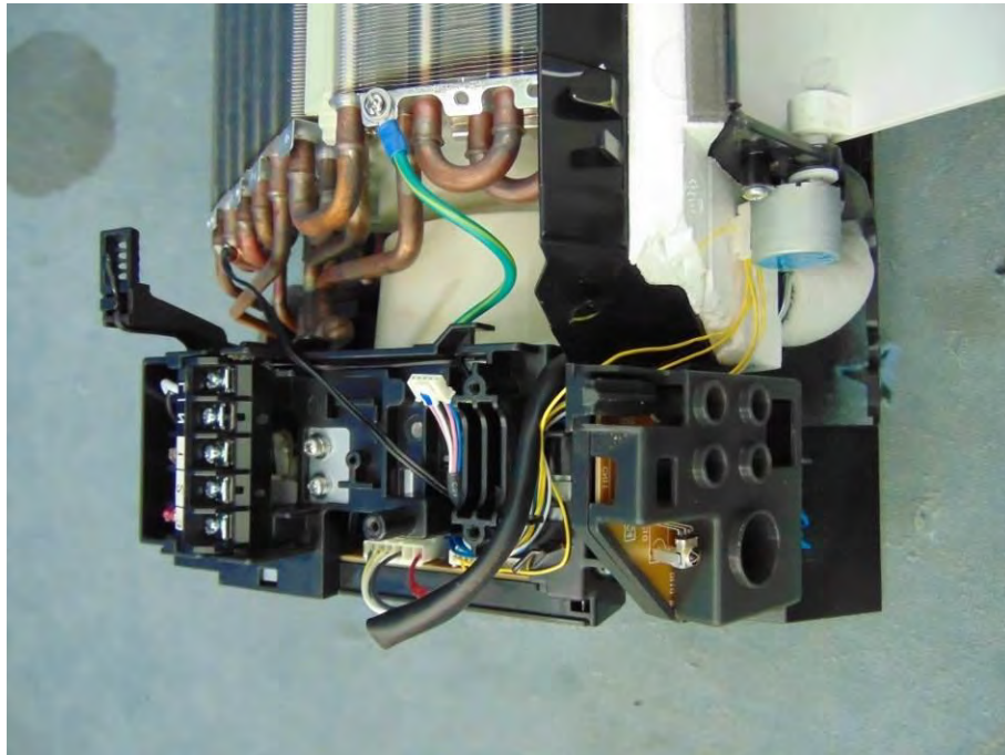
Picture No.64: Terminal view of indoor unit model: RAS-24PKVSG-EE
