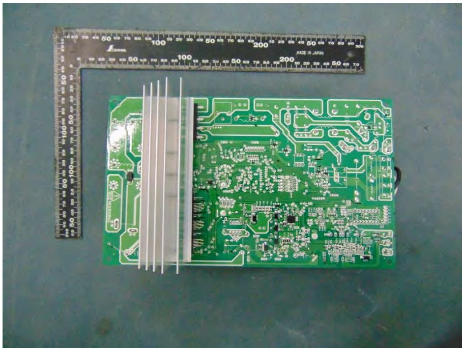
Picture No.73: Pattern view of PCB model: WP-048
