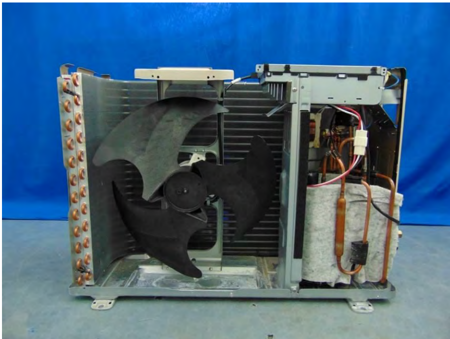
Picture No.18: Inner view of outdoor unit model: RAS-22J2AVRG-E
