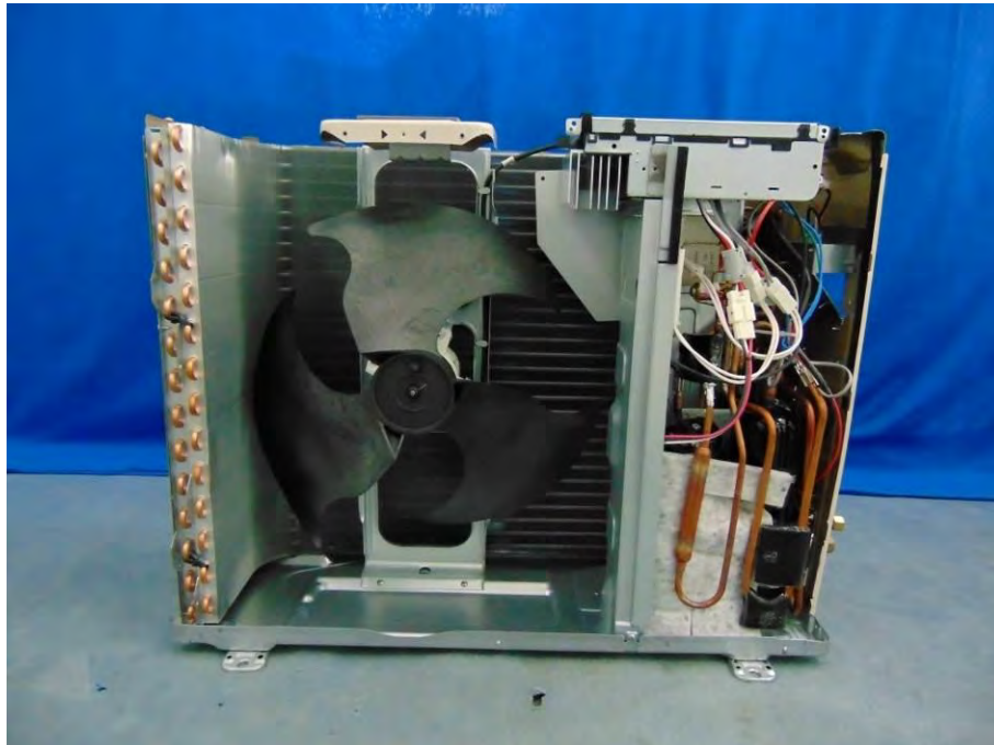
Picture No.25: Inner view of outdoor unit model: RAS-24J2AVRG-E
