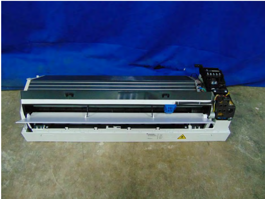
Picture No.44: Overall inner view of indoor unit model: RAS-B16J2KVRG-E
