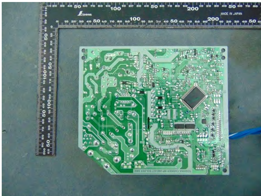
Picture No.71: Pattern view of PCB model: WP-048
