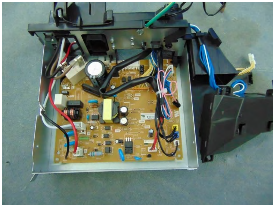
Picture No.59: PCB. compartment of indoor unit: RAS-B24J2KVRG-E
