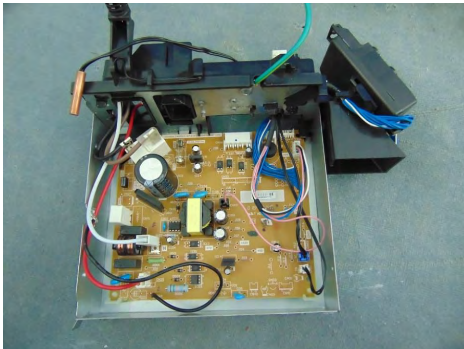
Picture No.65: PCB. compartment of indoor unit: RAS-24PKVSG-EE
