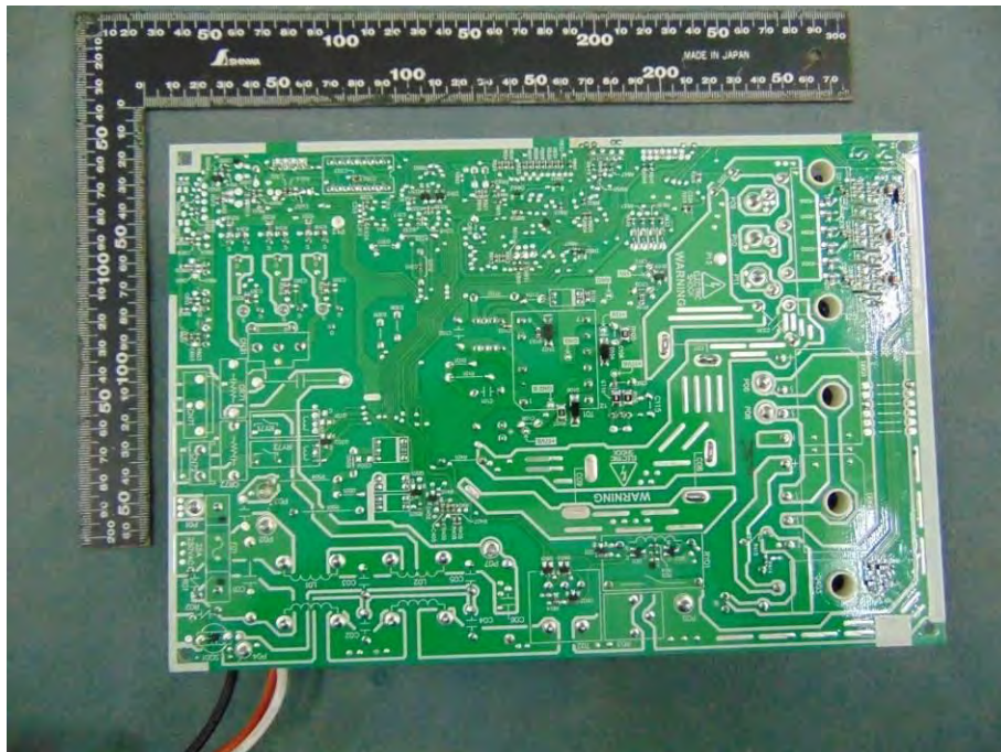
Picture No.69: Pattern view of PCB model: WP-030
