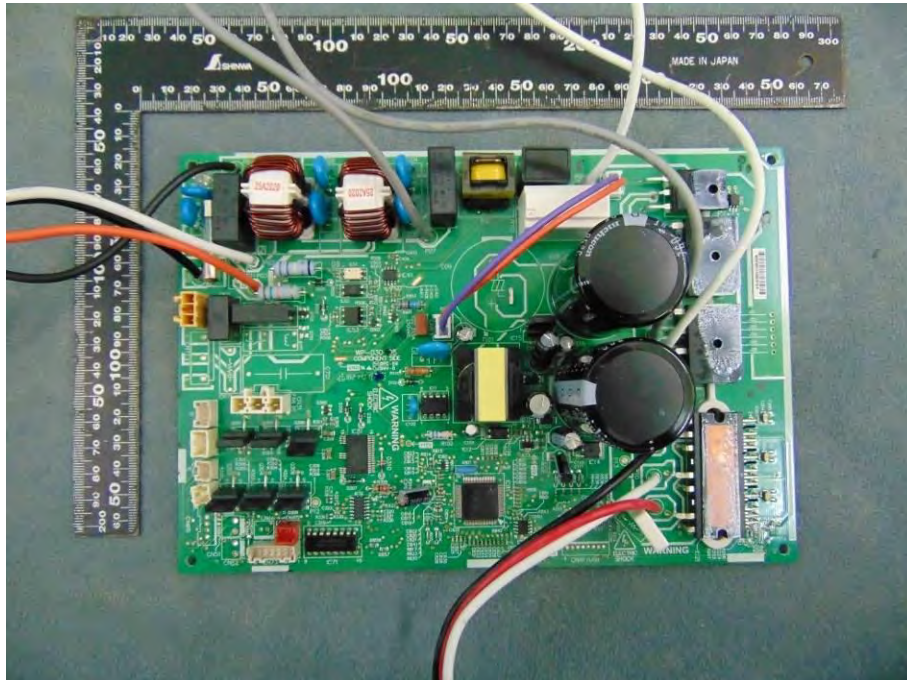
Picture No.68: Component view of PCB model: WP-030
