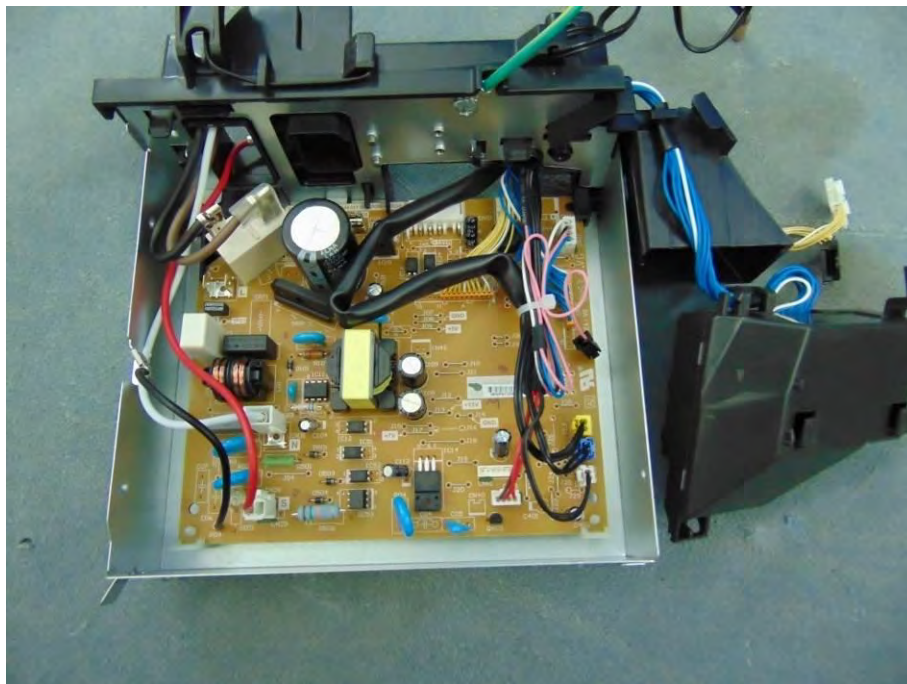
Picture No.47: PCB. compartment of indoor unit: RAS-B16J2KVRG-E
