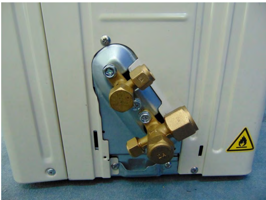
Picture No.24: Inner view of outdoor unit model: RAS-24J2AVRG-E
