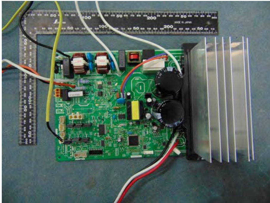
Picture No.27: Component view of PCB model: WP-030
