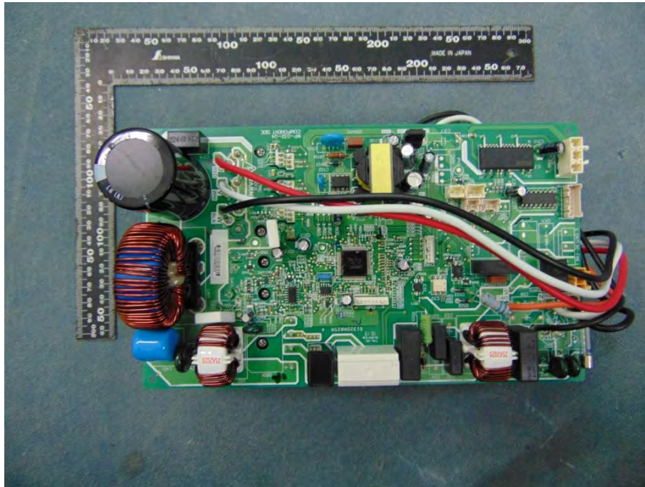
Picture No.13: Component view of PCB model: WP-032
