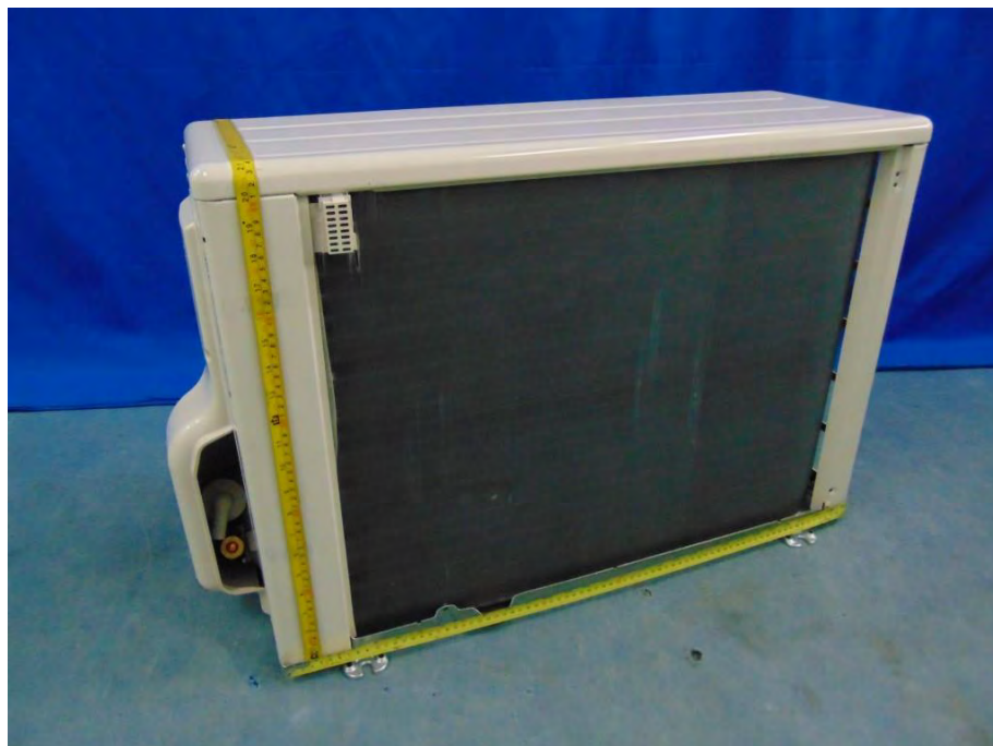
Picture No.16: Overall rear view of outdoor unit model: RAS-18TAVG-E
