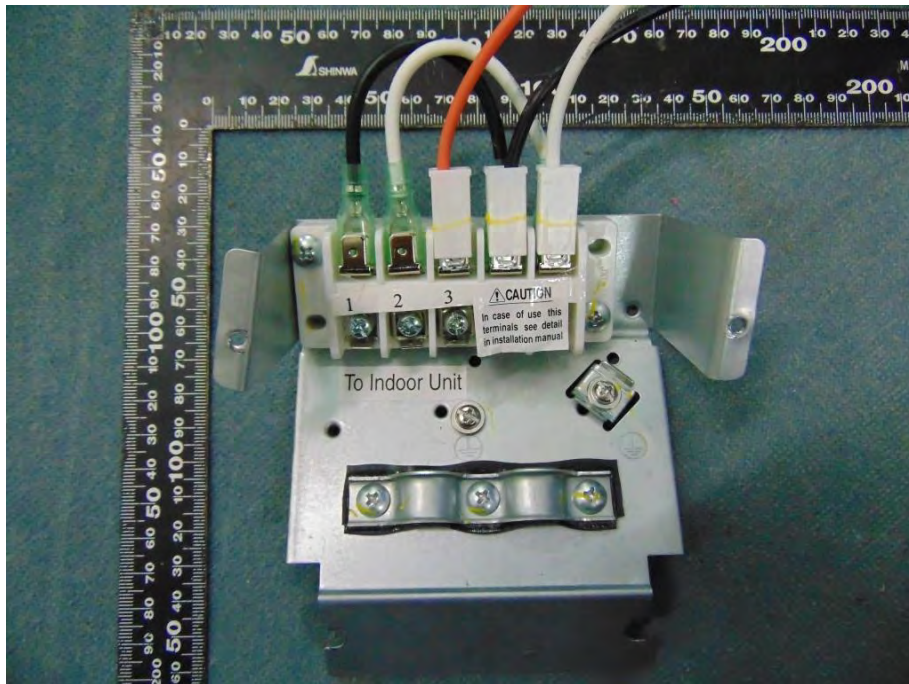
Picture No.19: Terminal of outdoor unit model: RAS-18TAVG-E
