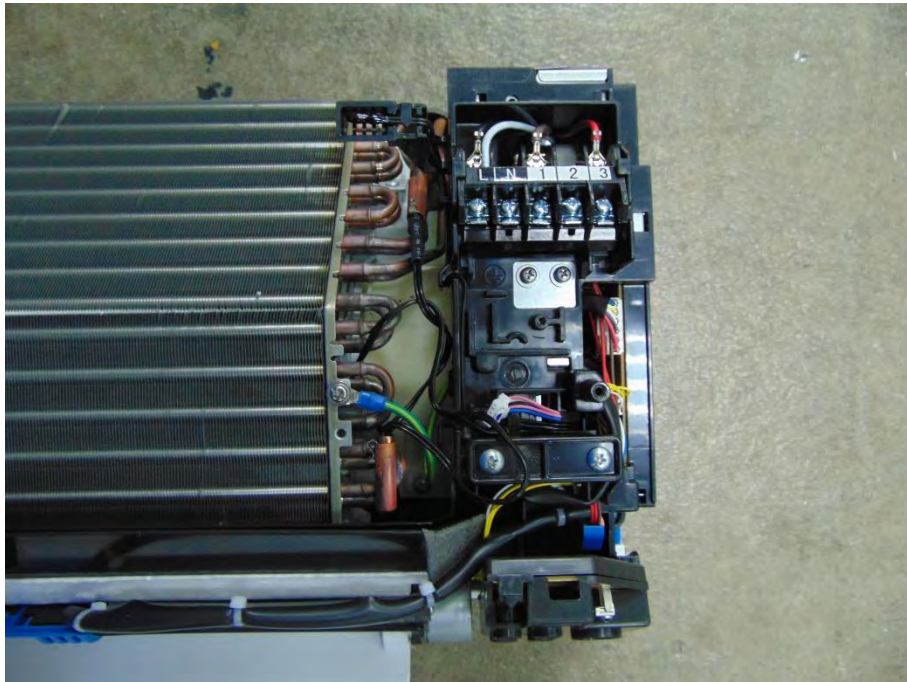
Picture No.33: Terminal view of indoor unit model: RAS-B10TKVG-E
