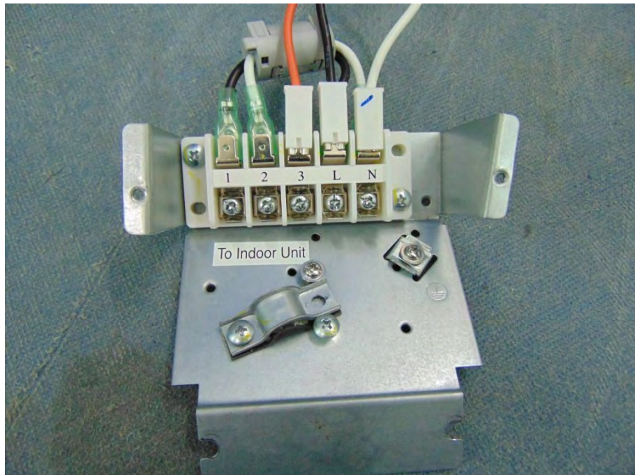
Picture No.11: Terminal of outdoor unit model: RAS-13TAVG-E
