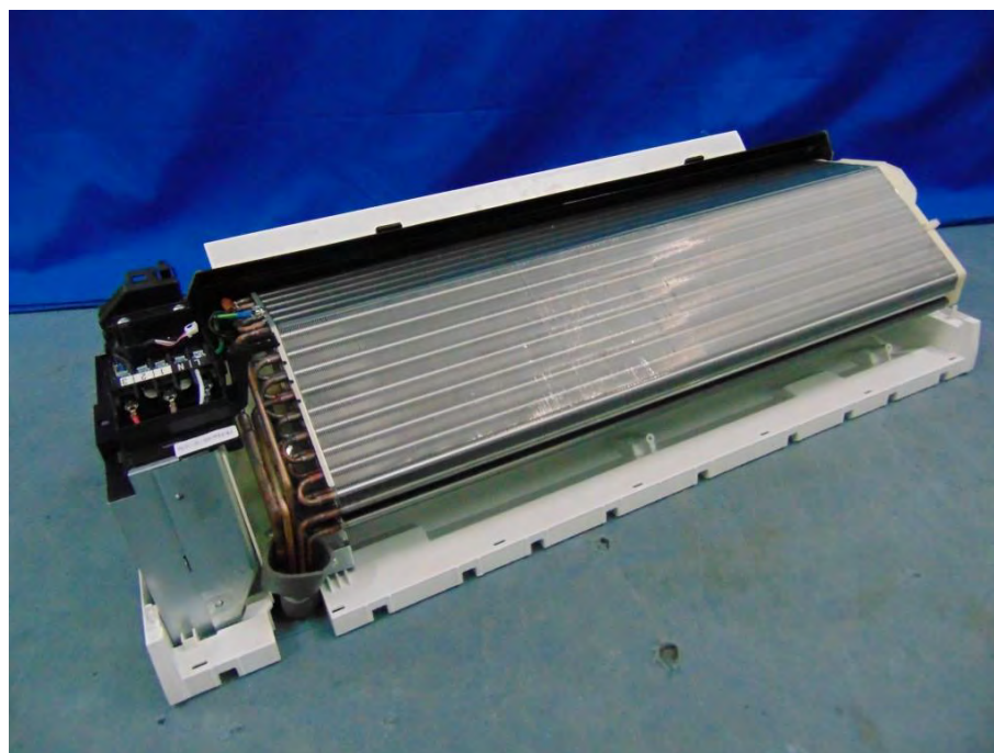
Picture No.44: Overall inner view of indoor unit model: RAS-18TKVG-E
