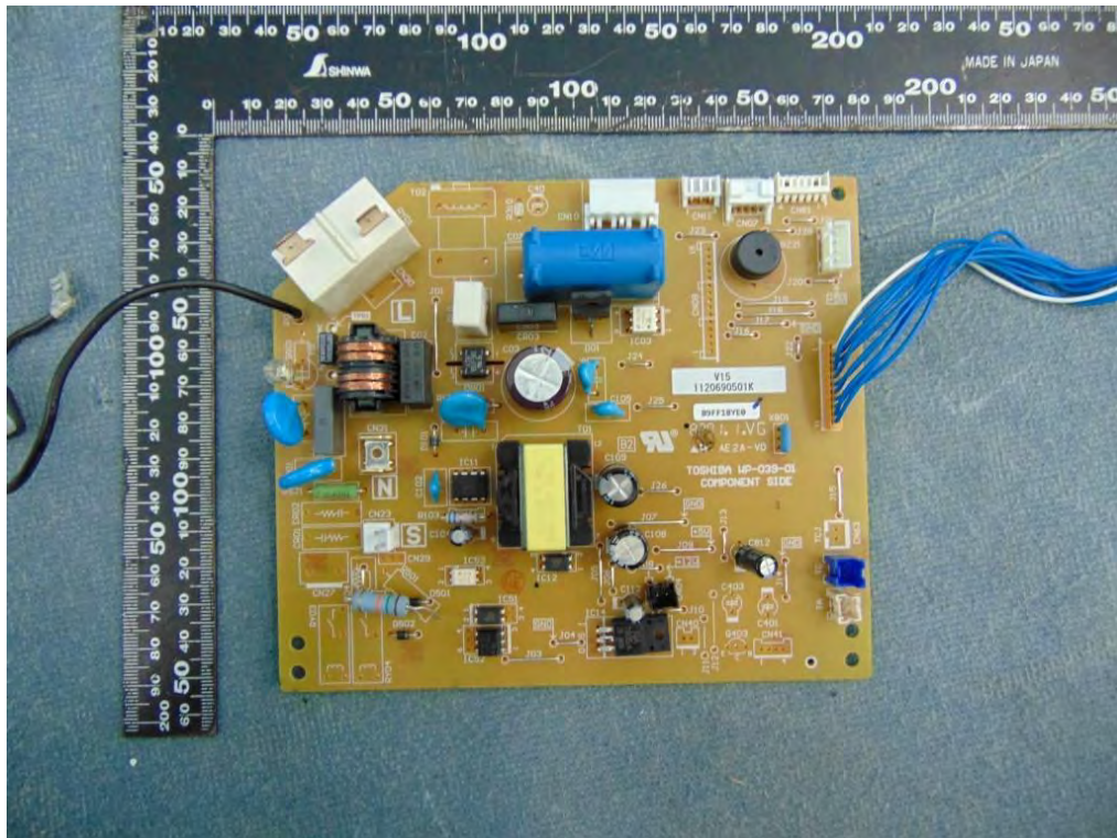
Picture No.39: Component view of PCB model: WP-039
