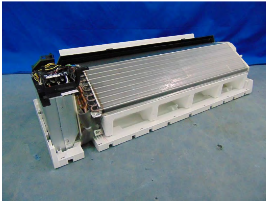
Picture No.37: Overall inner view of indoor unit model: RAS-B13TKVG-E
