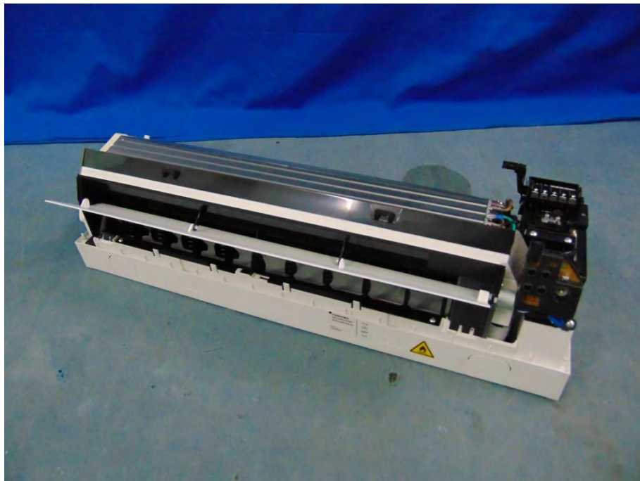
Picture No.43: Overall inner view of indoor unit model: RAS-18TKVG-E
