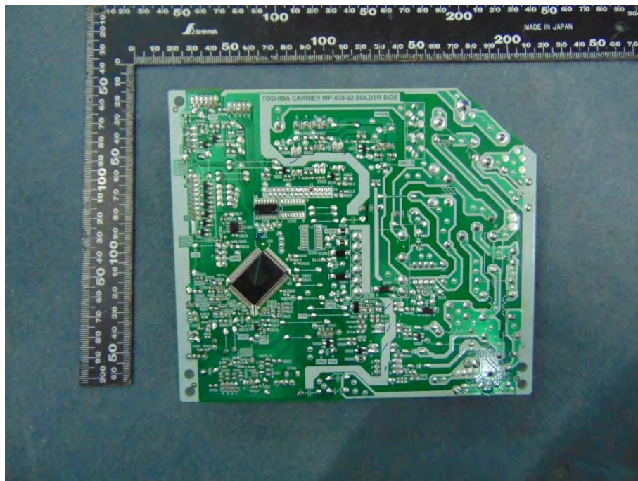
Picture No.52: Pattern view of PCB model: WP-038
