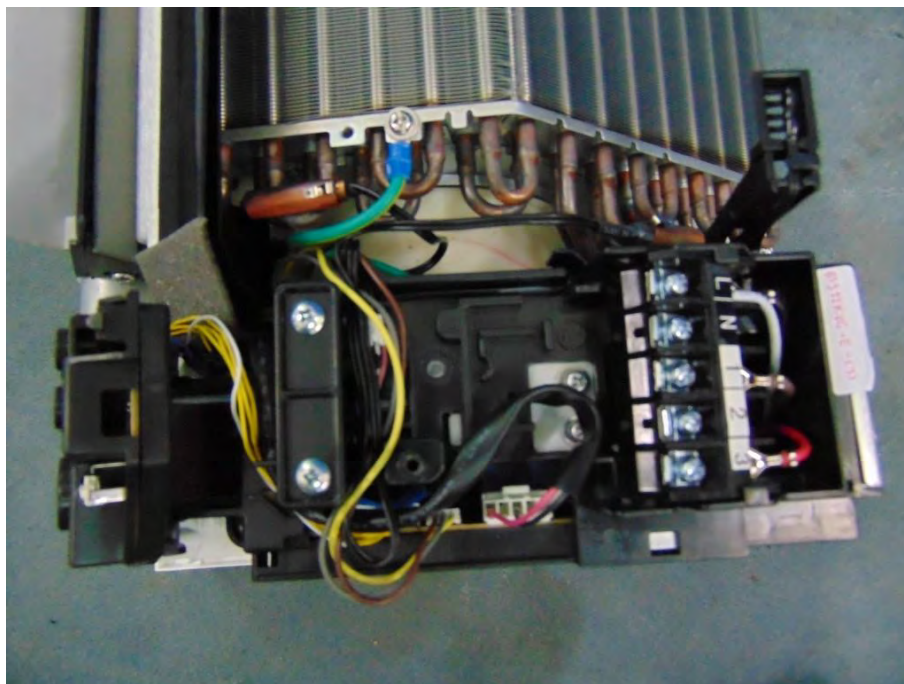
Picture No.38: Terminal view of indoor unit model: RAS-B13TKVG-E
