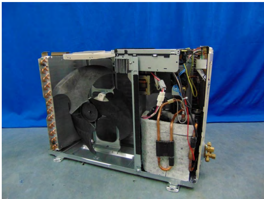
Picture No. 18: Inner side view of outdoor unit model: RAS-18TAVG-E
