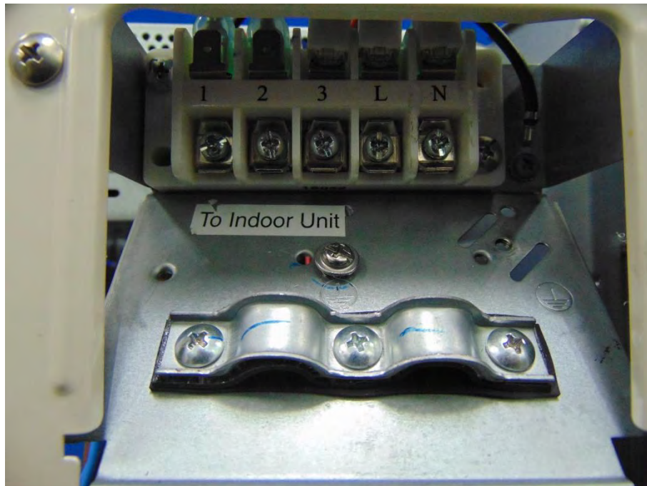
Picture No.5: Terminal of outdoor unit model: RAS-10TAVG-E
