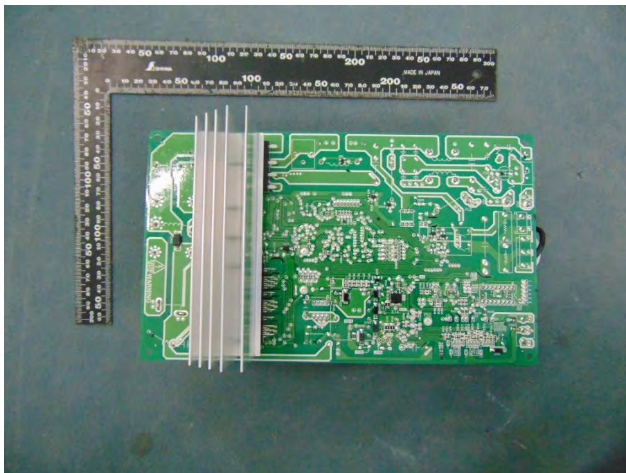
Picture No.14: Pattern view of PCB model: WP-032
