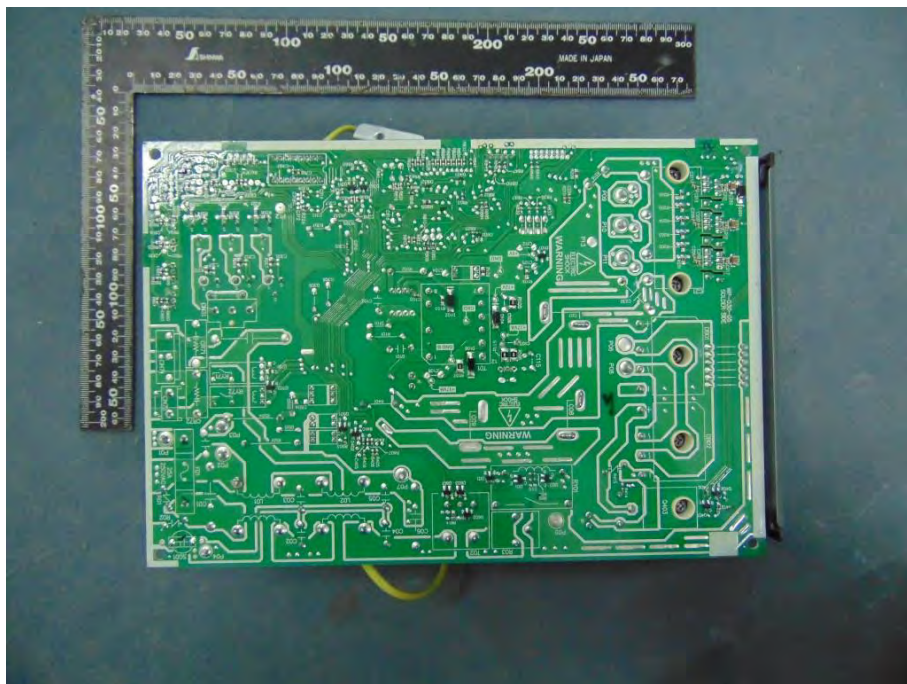
Picture No.28: Pattern view of PCB model: WP-030
