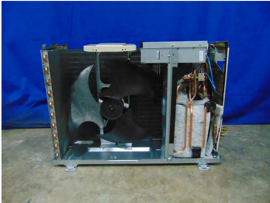
Picture No.3: Inner view of outdoor unit model: RAS-10TAVG-E
