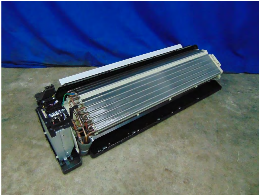
Picture No.49: Overall inner view of indoor unit model: RAS-24TKVG-E
