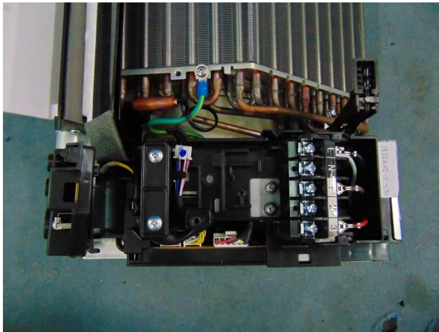
Picture No.45: Terminal view of indoor unit model: RAS-18TKVG-E
