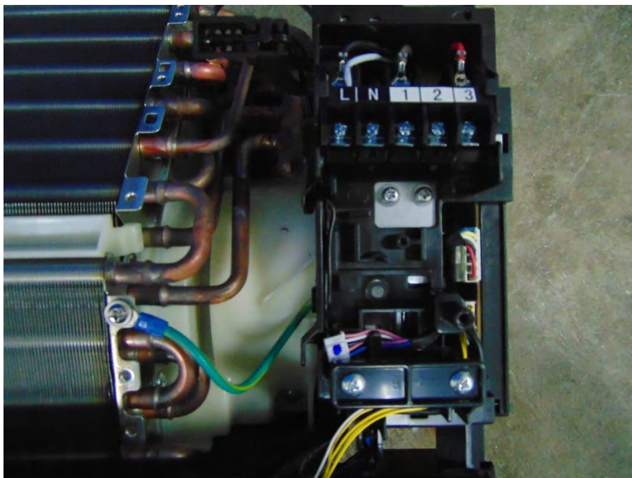
Picture No.50: Terminal view of indoor unit model: RAS-24TKVG-E
