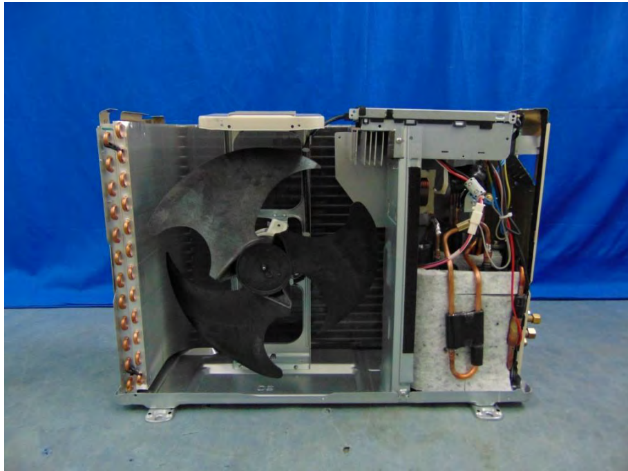
Picture No.17: Inner view of outdoor unit model: RAS-18TAVG-E
