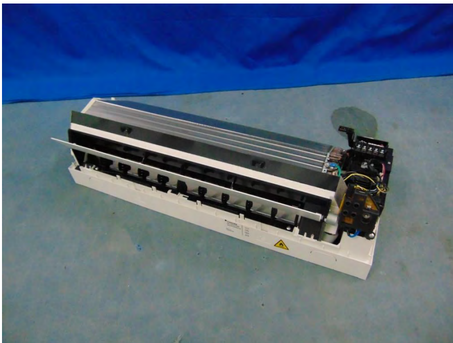
Picture No.36: Overall inner view of indoor unit model: RAS-B13TKVG-E
