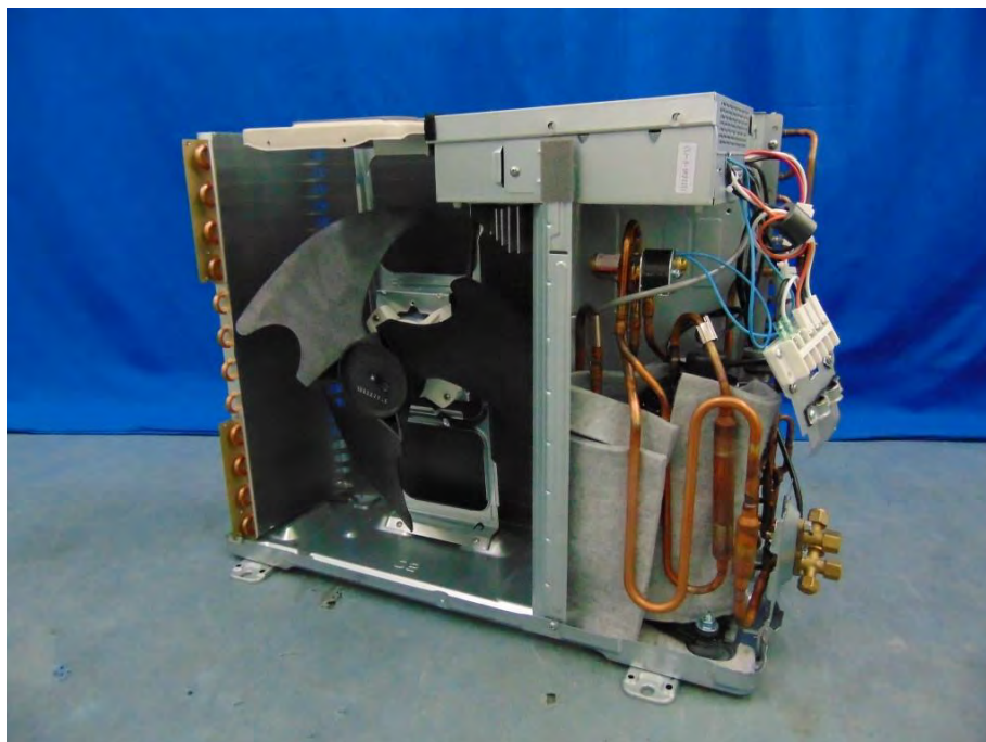
Picture No. 10: Inner side view of outdoor unit model: RAS-13TAVG-E
