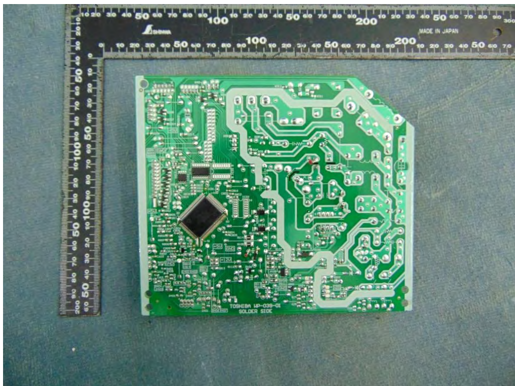
Picture No.40: Pattern view of PCB model: WP-039
