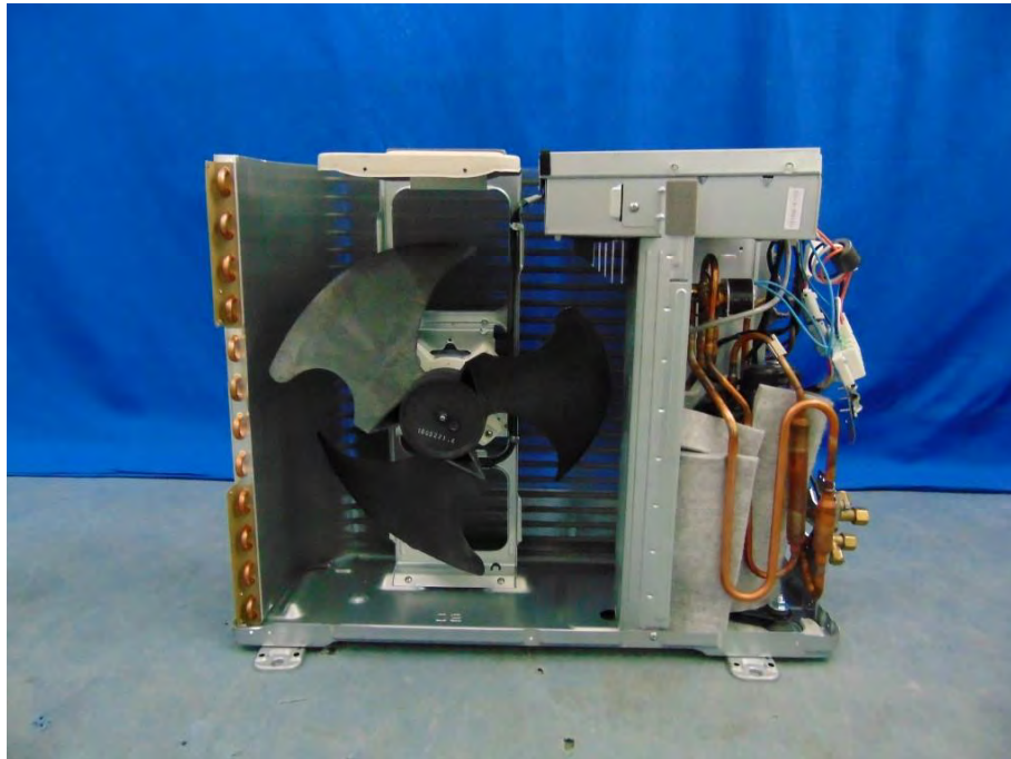
Picture No.9: Inner view of outdoor unit model: RAS-13TAVG-E
